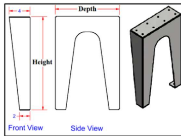
Mounting Bracket
